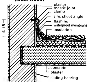
10 Wall connection zinc sheet angle and flashing
